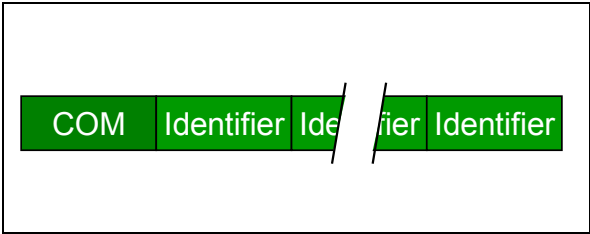
Figure 2-31: Ordered-Set Structure
