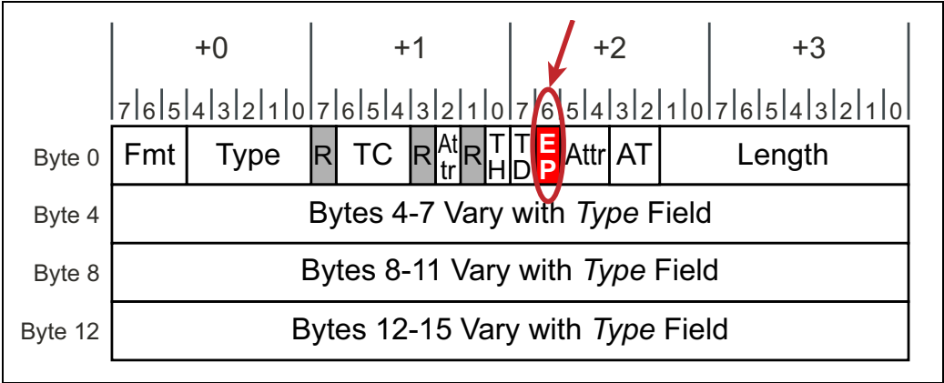
Figure 15-6: The Error/Poisoned Bit in a Completion Header
