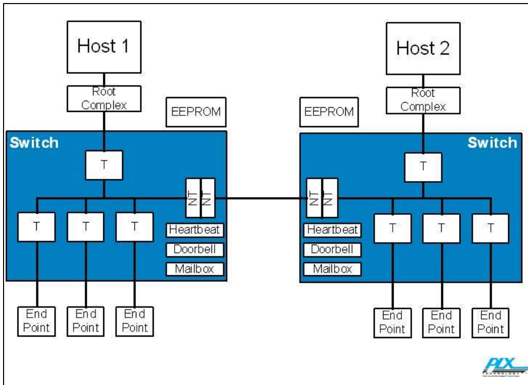
Figure 0-6: Dual Host in a PCI and PCI Express System
