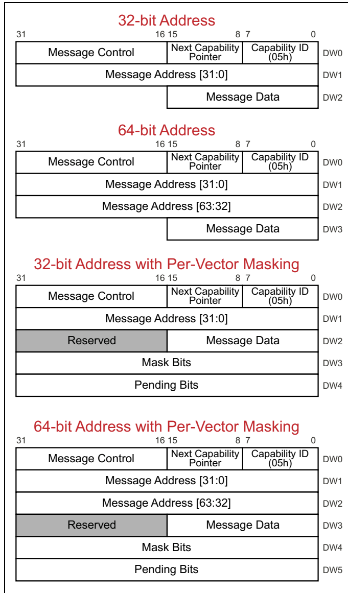
Figure 17-13: MSI Capability Structure Variations
